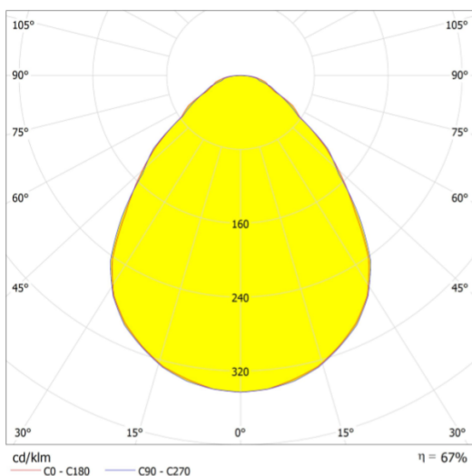
GDS Reality Series HELFLM Square Surface 590mm 3000K 35W Microprism / LDC (Polar)
